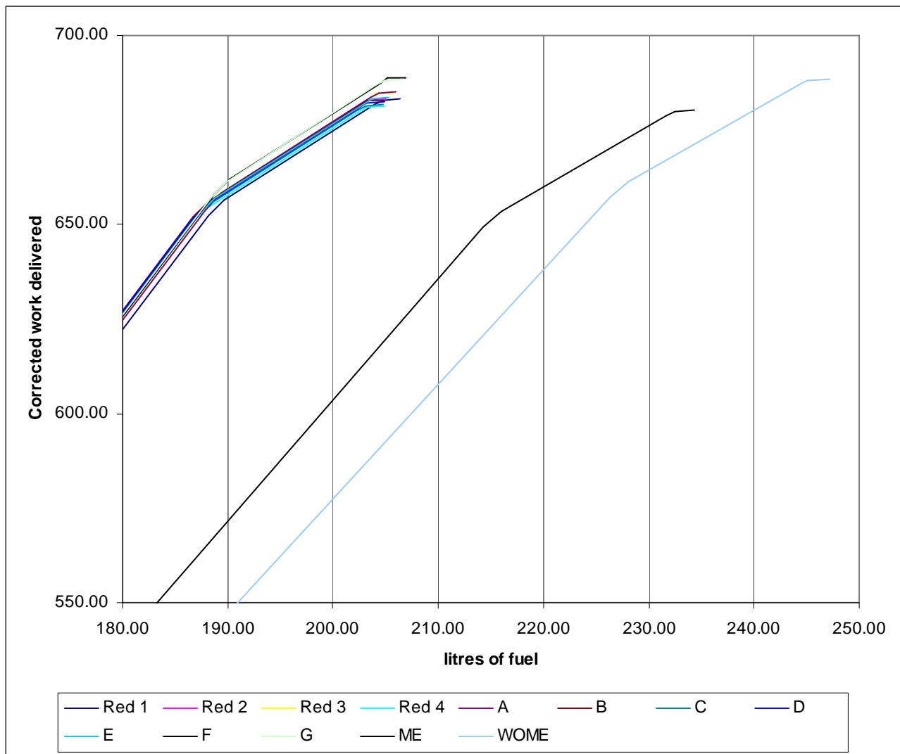
Figure 09: Comparison between fuel / fuel + additive cumulative performance over the DayTrawl test cycle. Corrected work delivered (kWh). Red X: DayTrawl test cycle with red diesel only. A – G: DayTrawl test cycle with red diesel and fuel additives A to G. ME: DayTrawl test cycle with BS 14214 methyl ester. WOME: DayTrawl test cycle with Waste Oil Methyl Ester (WOME).
